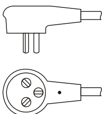
Israeli plug 10/16A / 250V with 3 pins
