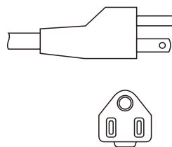
USA - Canada 5-15A / 120V earthed (UL approved)
