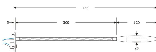
SIDE ELEVATION
